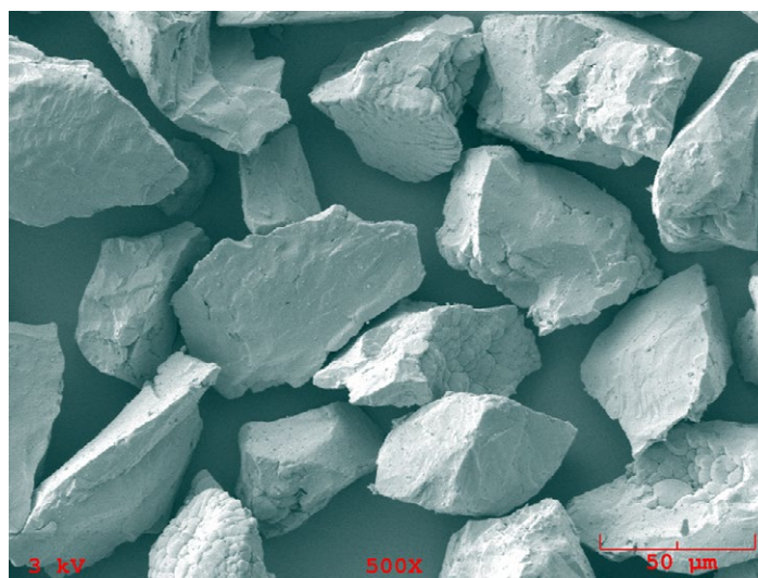
Photomicrograph of typical fused and crushed morphology for these materials
