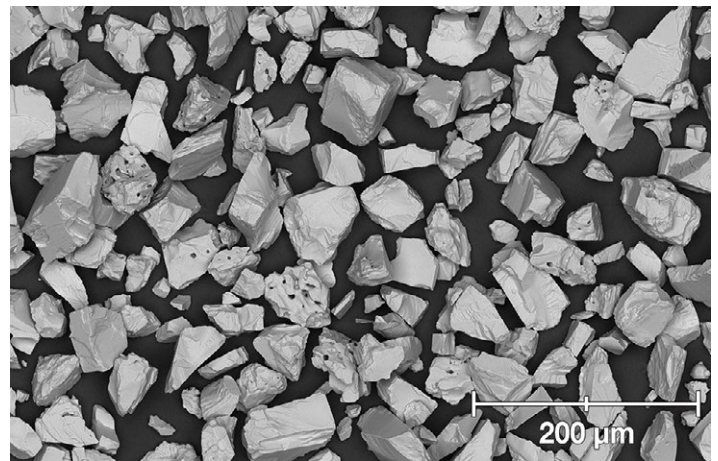
SEM photomicrograph showing the typical morphology of these materials
