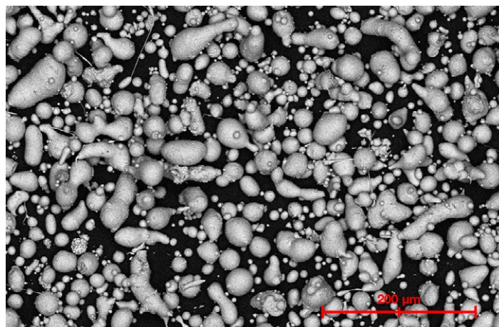
SEM photomicrograph morphology of Diamalloy 1008 (top)
