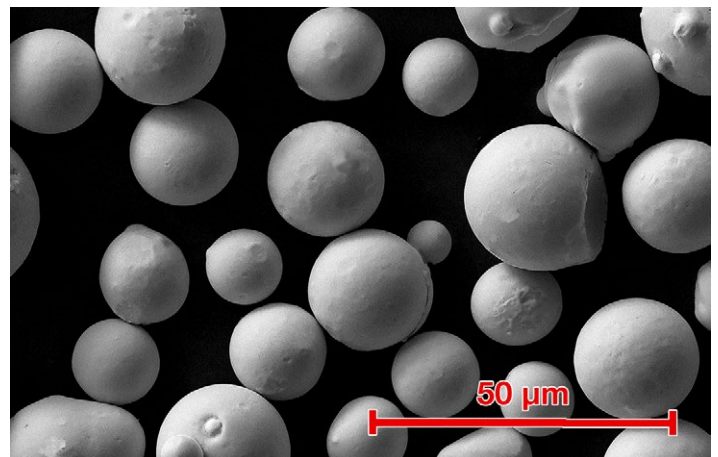
Typical morphology of MetcoAdd MM509-A gas atomized powder for additive manufacturing.
