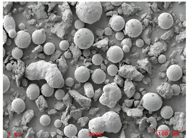
Morphology of Metco 439NS powder blend
