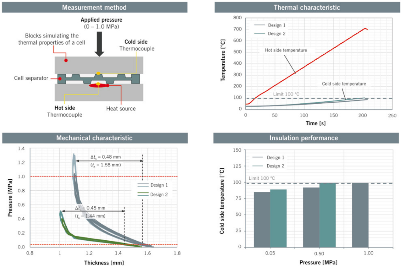
FIGURE 6 Thermal and mechanical characteristics of a multi-functional cell separator (© Oerlikon)
