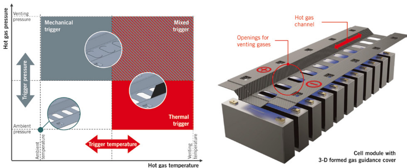
FIGURE 4 Trigger options for venting openings of gas guiding elements (© Oerlikon)
