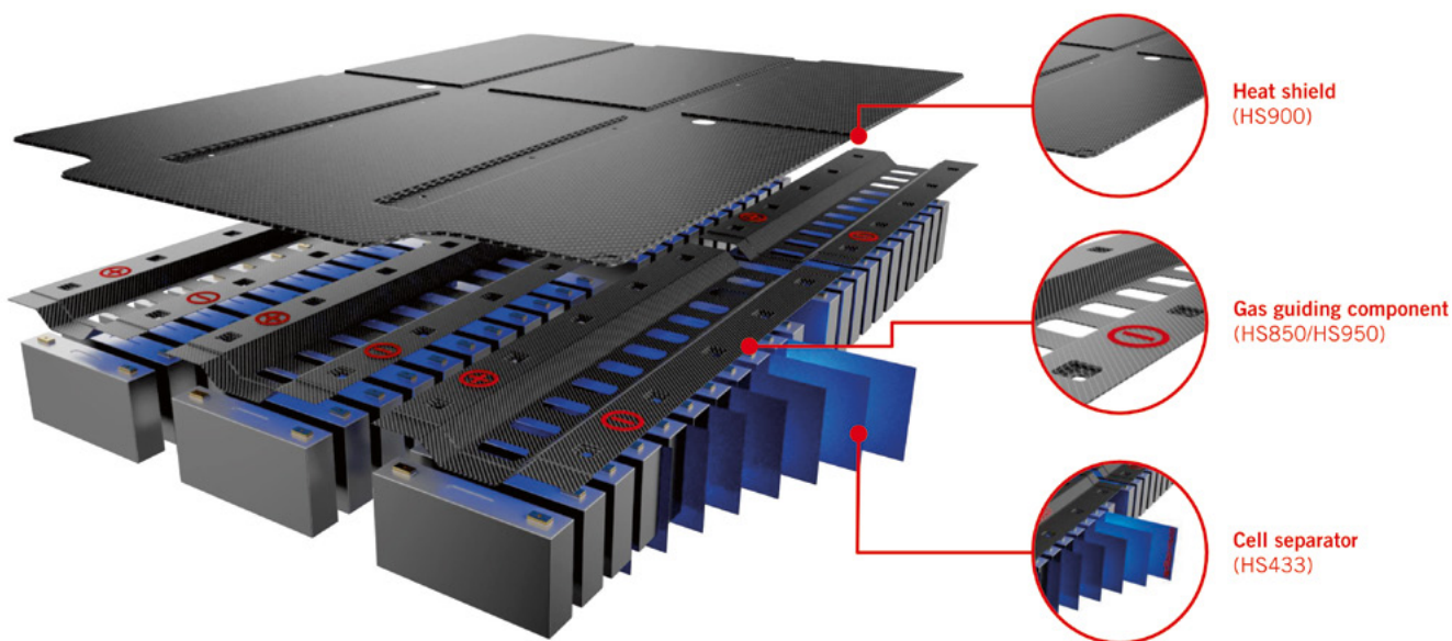
FIGURE 1 Heat resistant components for safety concepts of battery electric vehicles (© Oerlikon)
